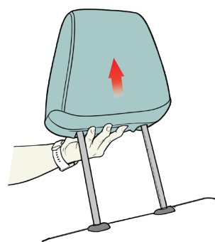
Release the headrest locking button, then remove the headrest.
